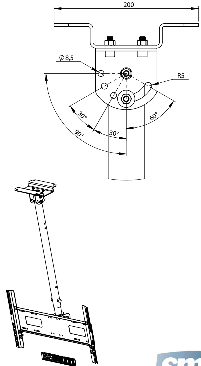
DETAIL A SCALE 1 : 3
