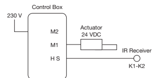
13 WIRING DIAGRAM
